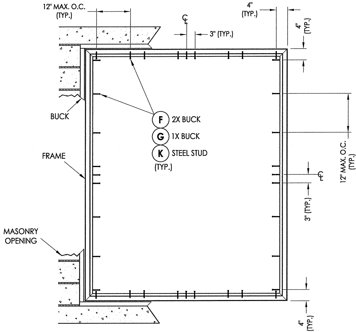
FRAME ANCHORING
