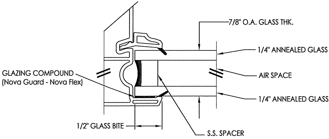
G3 GLAZING DETAIL
