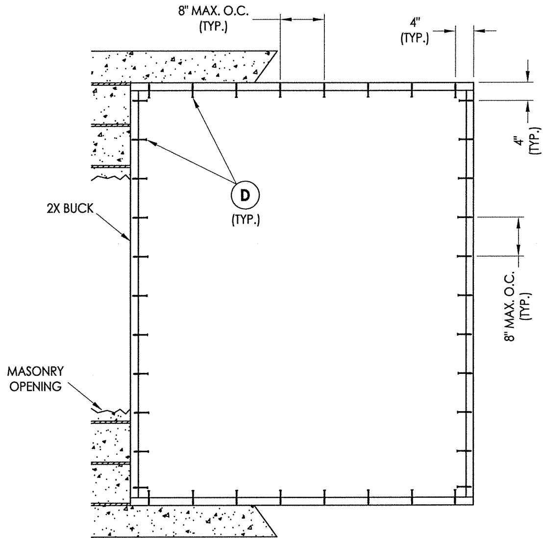
BUCK ANCHORING
